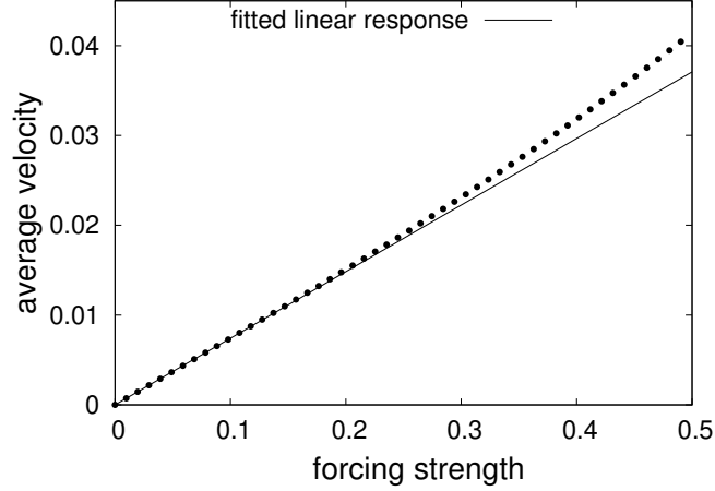
Fig. 8.2. Linear response of the numerical approximation of the average velocity \mathbb{E}_\eta(F^T M^{-1} p) as a function of \eta for the scheme associated with P_{\Delta t}^{\gamma C, B_\eta, A, B_\eta, \gamma C} , for \Delta t = 0.01 and \gamma = 1 . A linear fit on the first ten values gives a slope of \rho_{F,\Delta t} \simeq 0.07416 .
