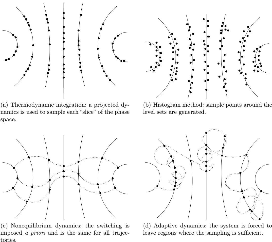
Fig. 7.7. Cartoon comparison of the different techniques to compute free energy differences in the reaction coordinate case.
